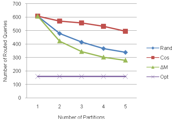
Figure 2. Number of queries routed to P (Q_r) with various partitioning techniques over various numbers of partitions.
